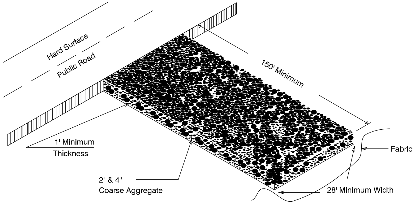
GRAVEL CONSTRUCTION ENTRANCE
