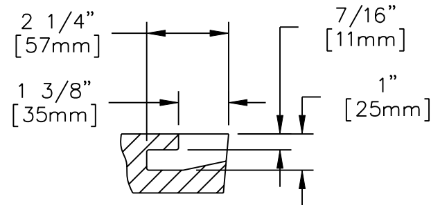
PICKHOLE DETAIL
