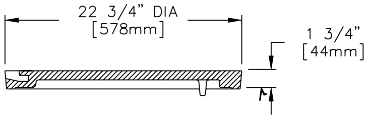
COVER SECTION
