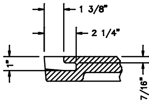
CONCEALED PICKHOLE DETAIL QUARTER SCALE
