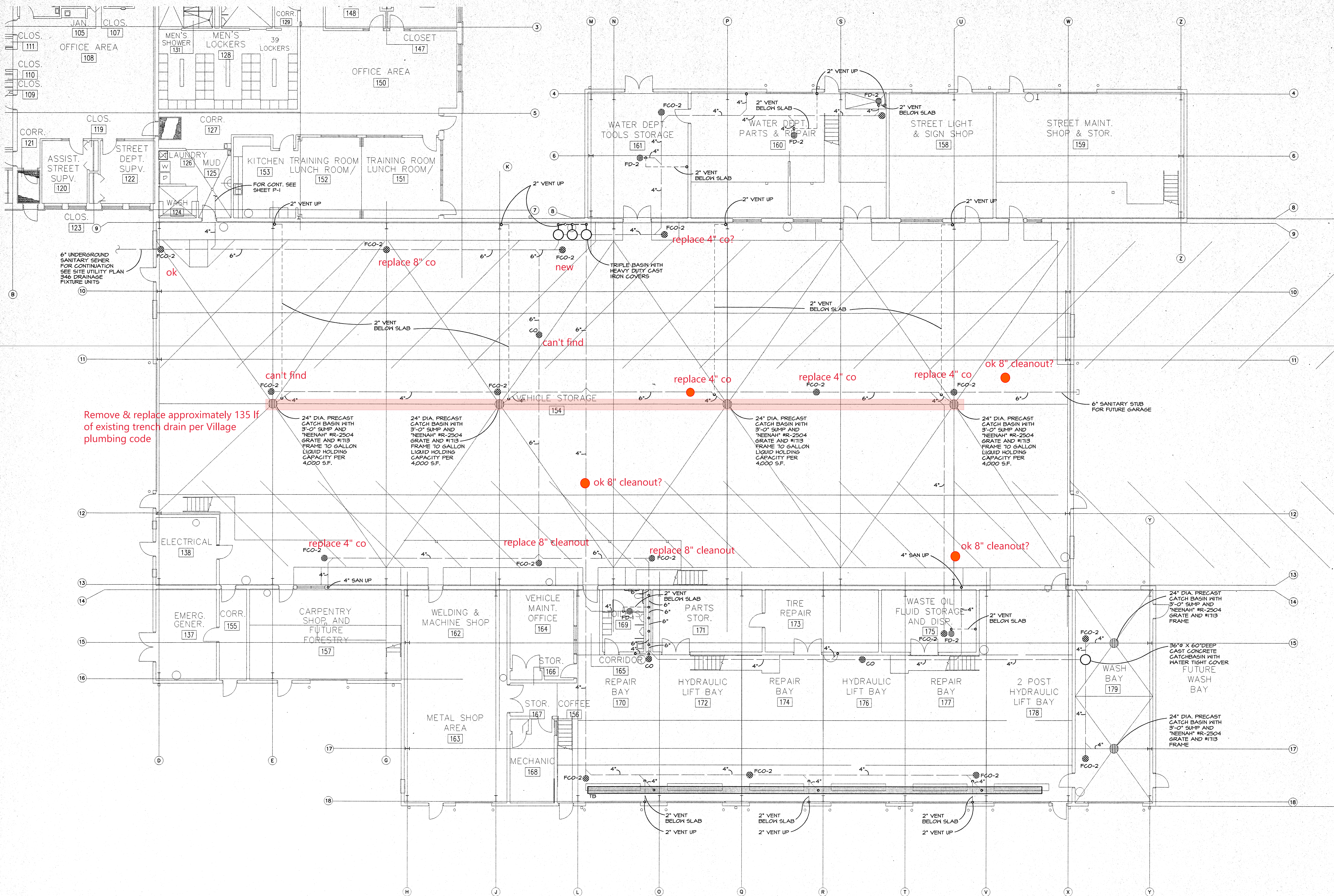
GARAGE PLUMBING PLAN
